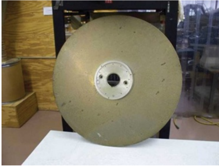
Figure A.3 One platter of that disk: 3/8 inch thick, 36 inches in diameter
